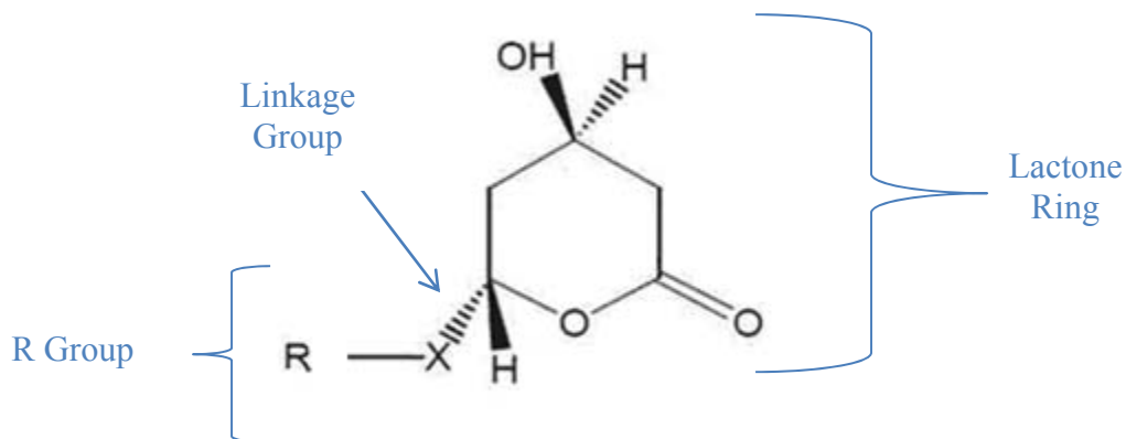
Figure 1: Generalized Structure of Statins 2
